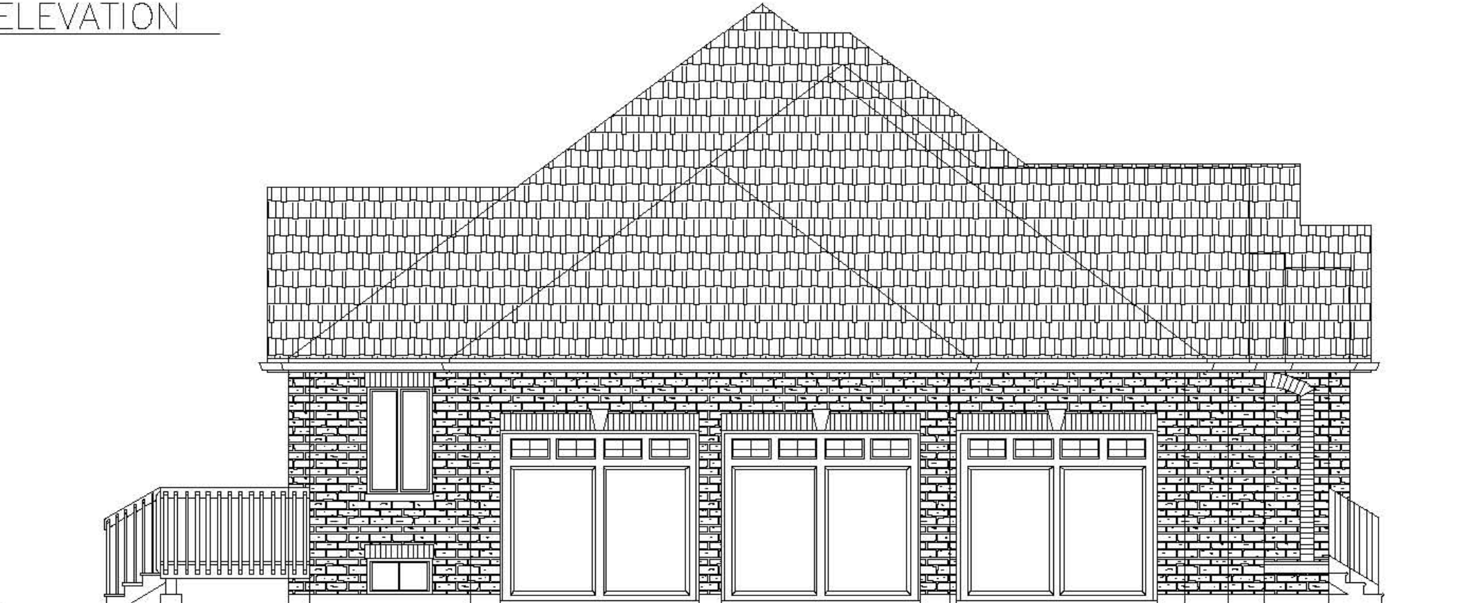
SIDE ELEVATION
